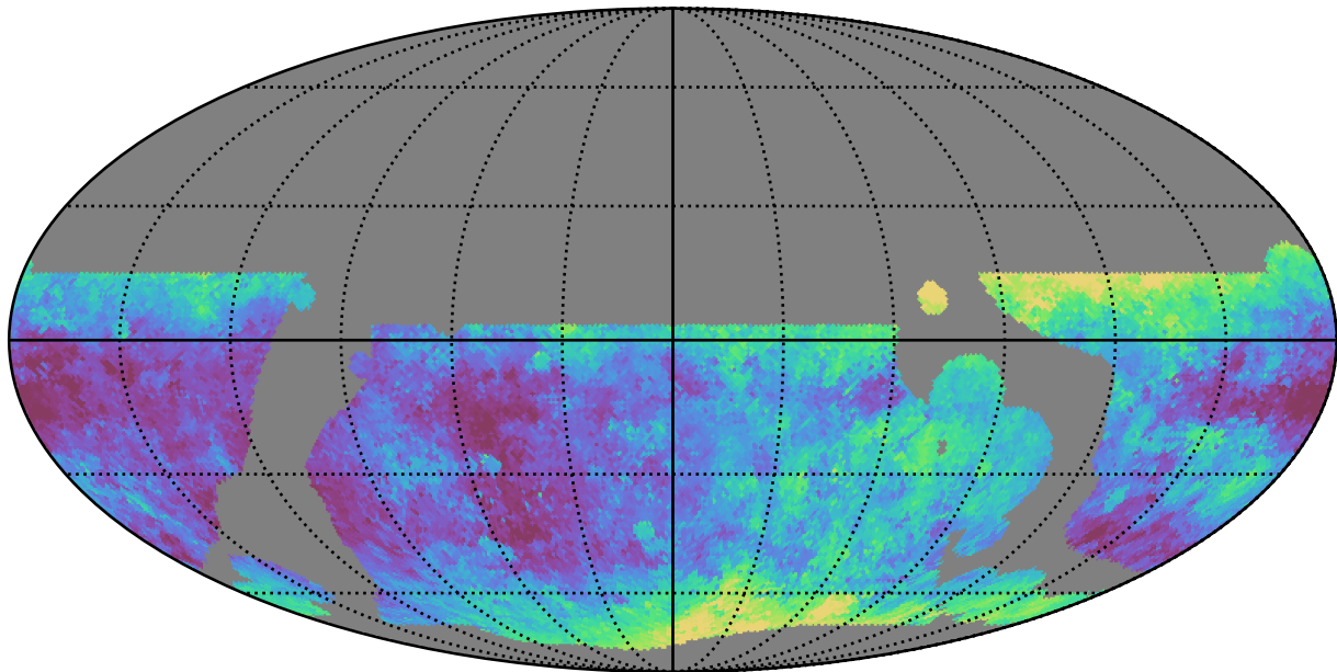
weather_cloudso0v3.5_10yrs WFD g band: Median seeingEff
