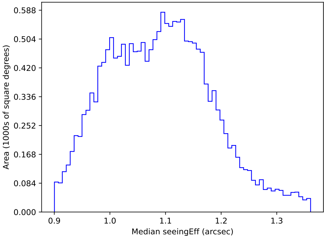
weather_cloudso0v3.5_10yrs WFD g band: Median seeingEff
