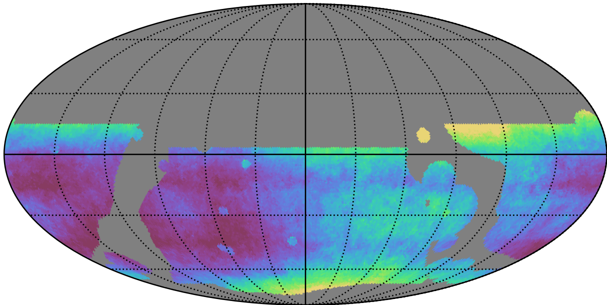
weather_cloudso0v3.5_10yrs WFD all bands: Median seeingEff
