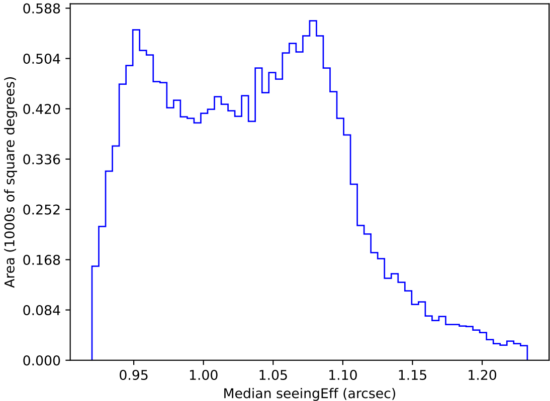
weather_cloudso0v3.5_10yrs WFD all bands: Median seeingEff
