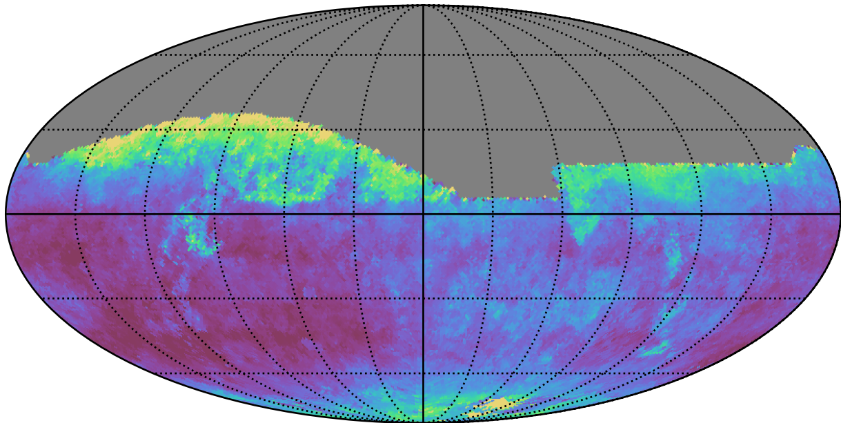
weather_cloudso0v3.5_10yrs All sky z band: Median seeingEff
