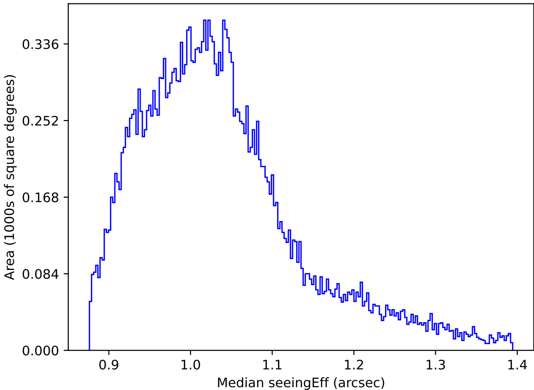
weather_cloudso0v3.5_10yrs All sky z band: Median seeingEff
