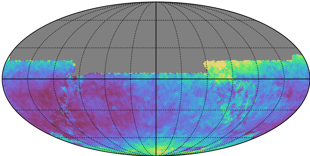
weather_cloudso0v3.5_10yrs All sky y band: Median seeingEff
