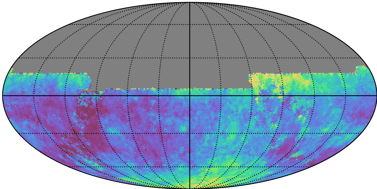
weather_cloudso0v3.5_10yrs All sky u band: Median seeingEff
