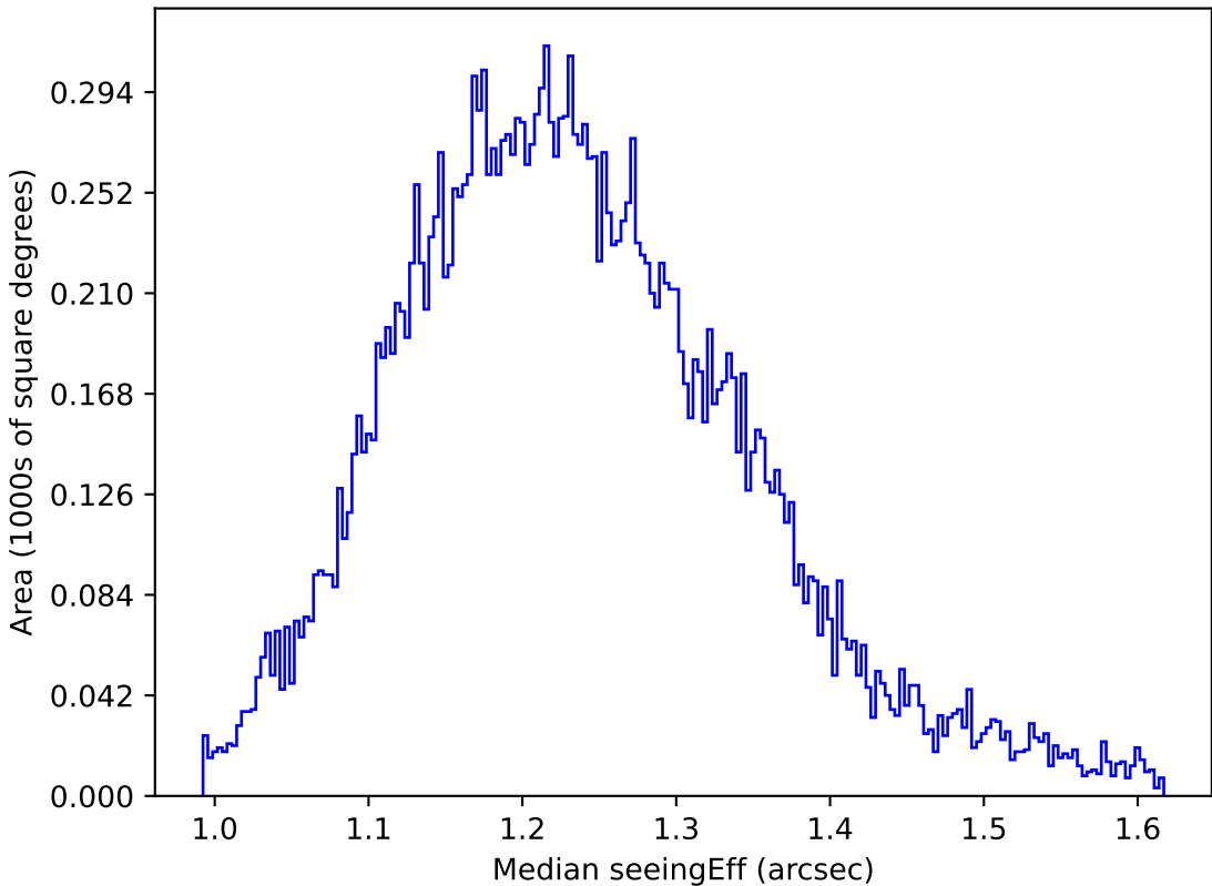
weather_cloudso0v3.5_10yrs All sky u band: Median seeingEff
