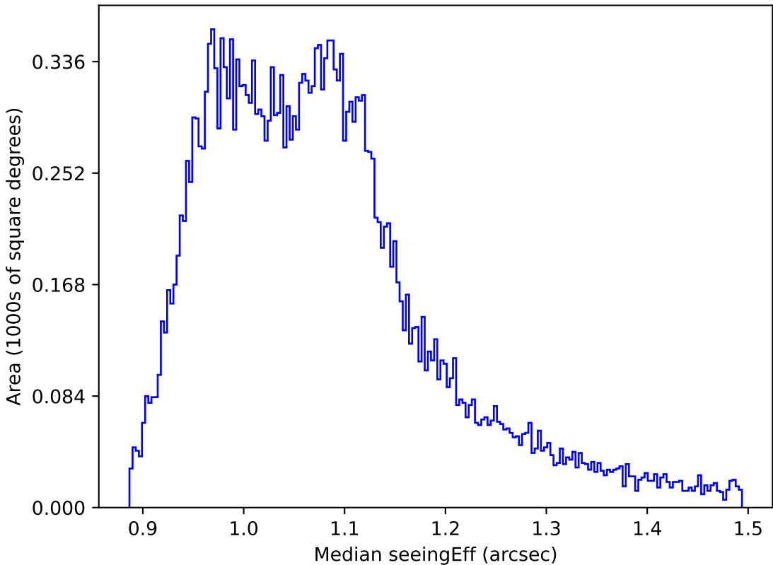
weather_cloudso0v3.5_10yrs All sky r band: Median seeingEff
