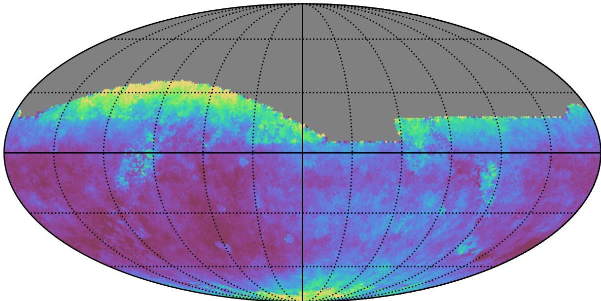
weather_cloudso0v3.5_10yrs All sky i band: Median seeingEff
