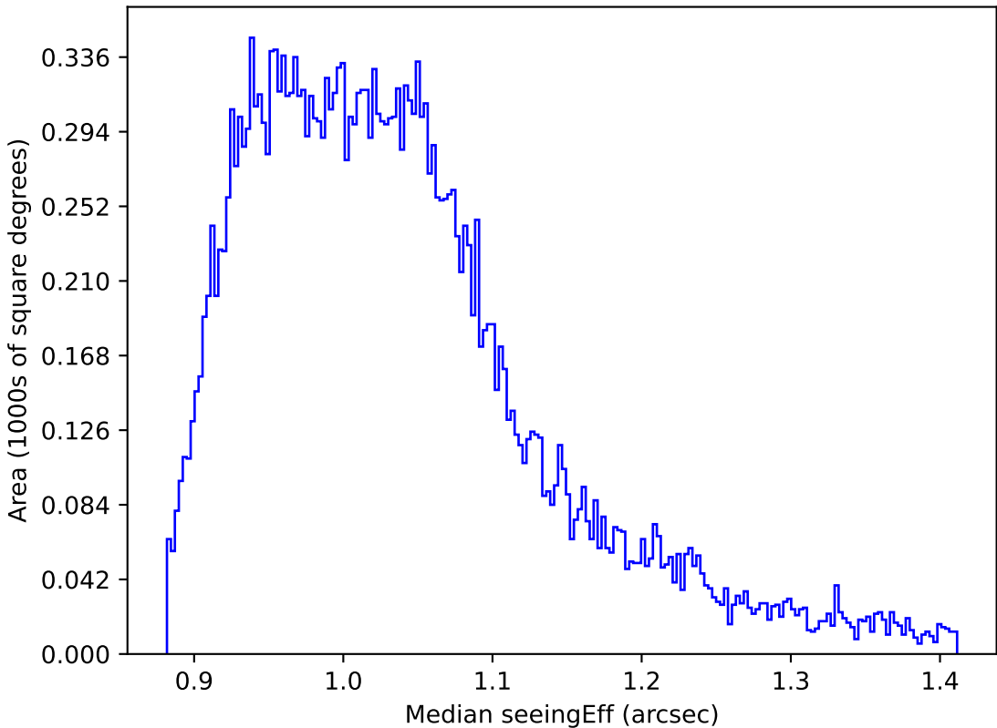
weather_cloudso0v3.5_10yrs All sky i band: Median seeingEff
