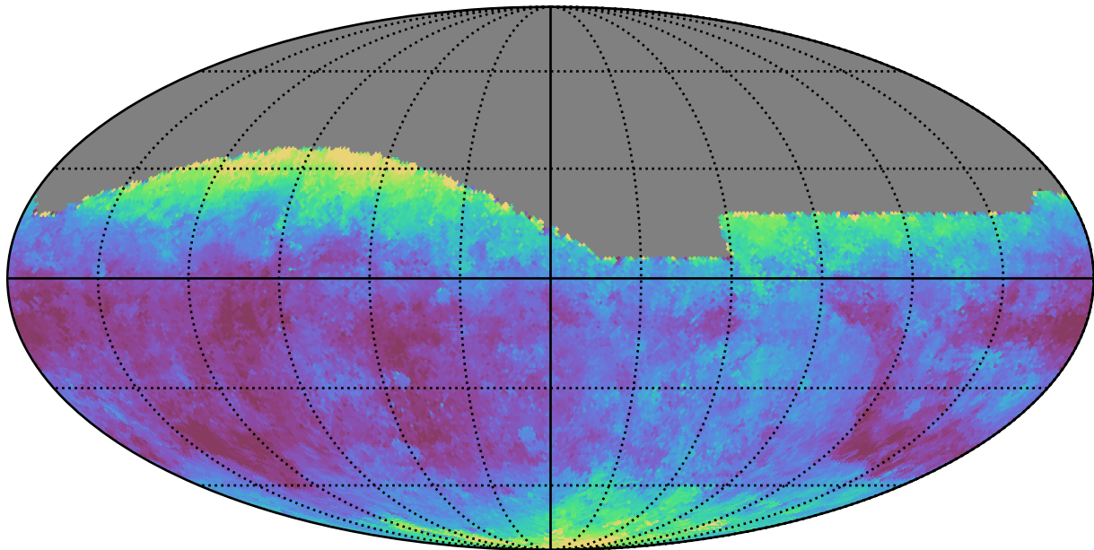
weather_cloudso0v3.5_10yrs All sky g band: Median seeingEff
