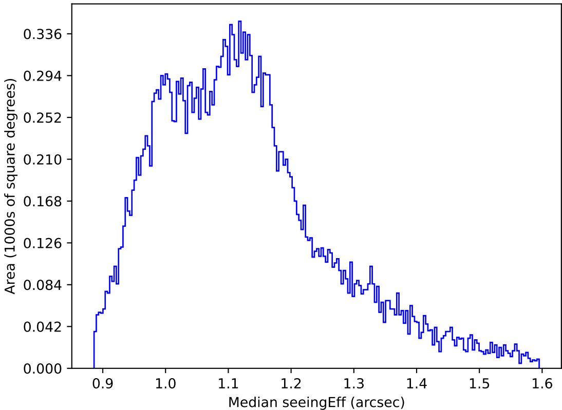
weather_cloudso0v3.5_10yrs All sky g band: Median seeingEff
