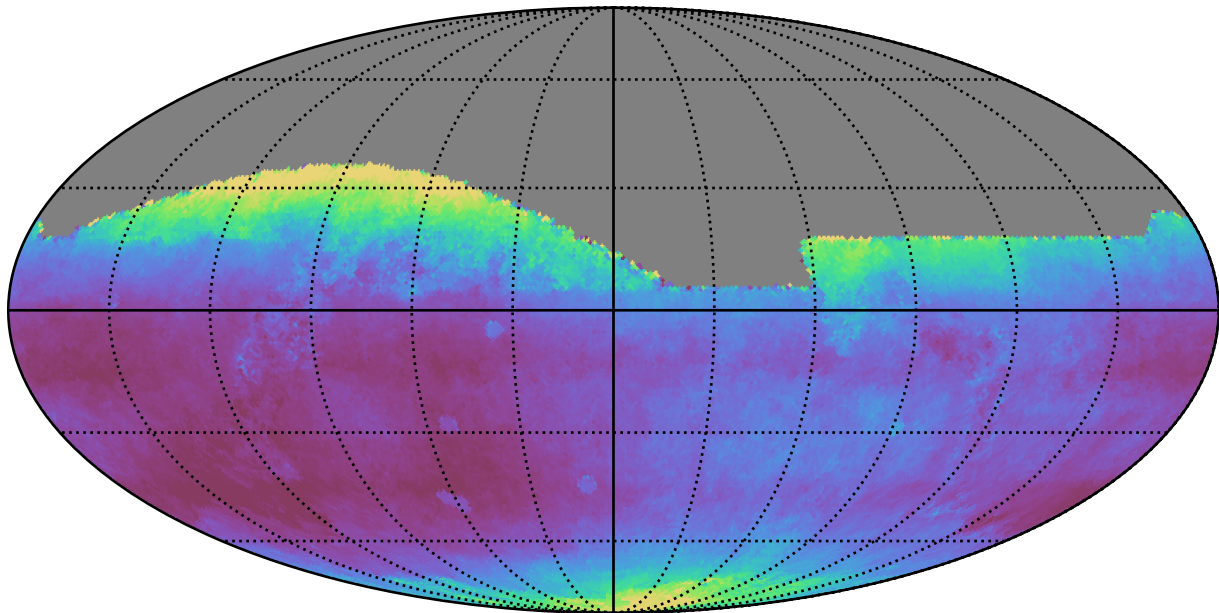
weather_cloudso0v3.5_10yrs All sky all bands: Median seeingEff
