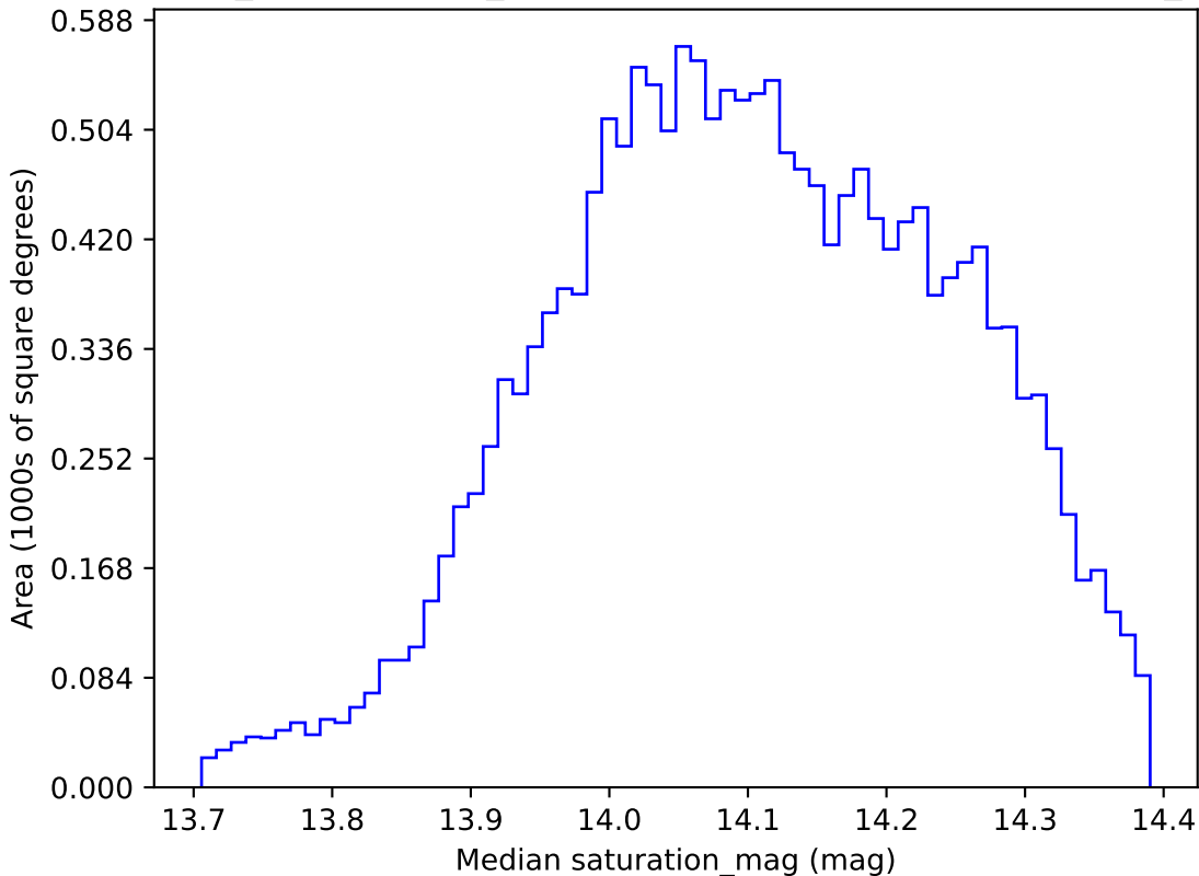
weather_cloudso0v3.5_10yrs WFD z band: Median saturation_mag
