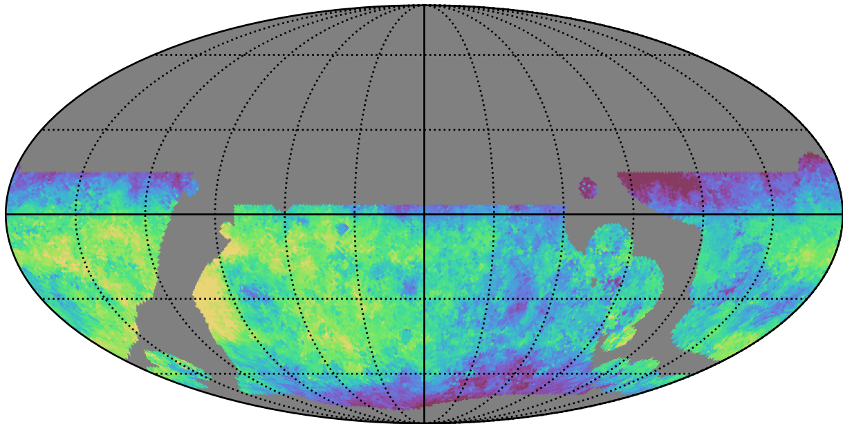
weather_cloudso0v3.5_10yrs WFD u band: Median saturation_mag
