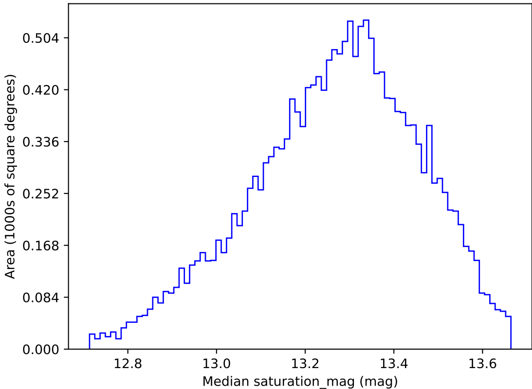
weather_cloudso0v3.5_10yrs WFD u band: Median saturation_mag
