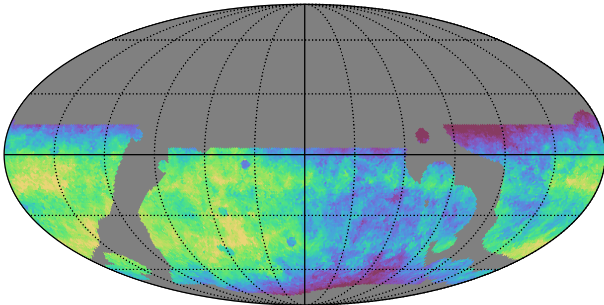
weather_cloudso0v3.5_10yrs WFD r band: Median saturation_mag
