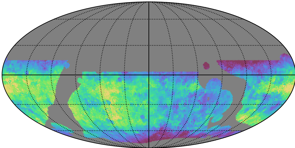
weather_cloudso0v3.5_10yrs WFD g band: Median saturation_mag
