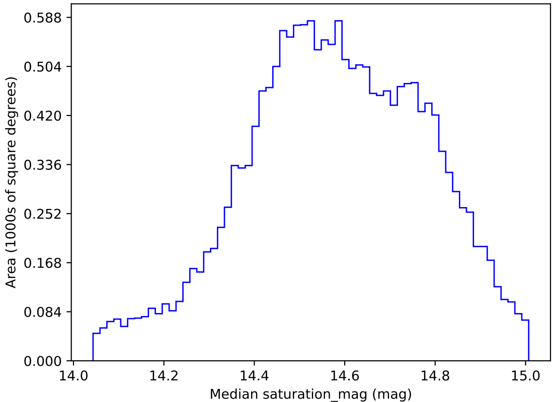
weather_cloudso0v3.5_10yrs WFD g band: Median saturation_mag
