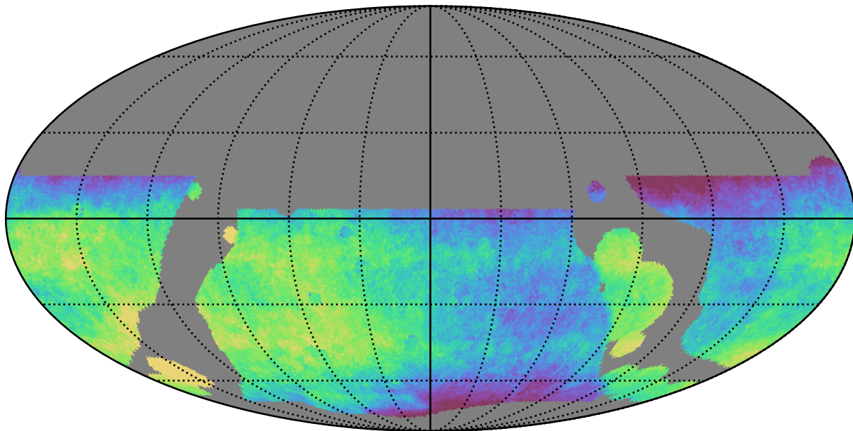
weather_cloudso0v3.5_10yrs WFD all bands: Median saturation_mag
