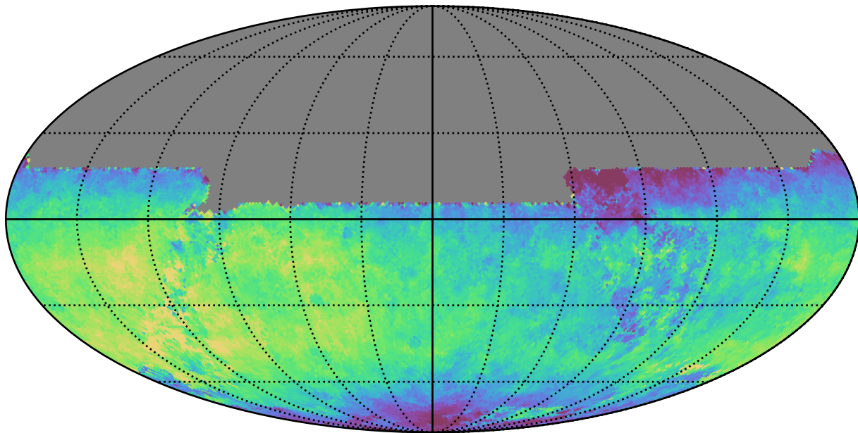
weather_cloudso0v3.5_10yrs All sky y band: Median saturation_mag
