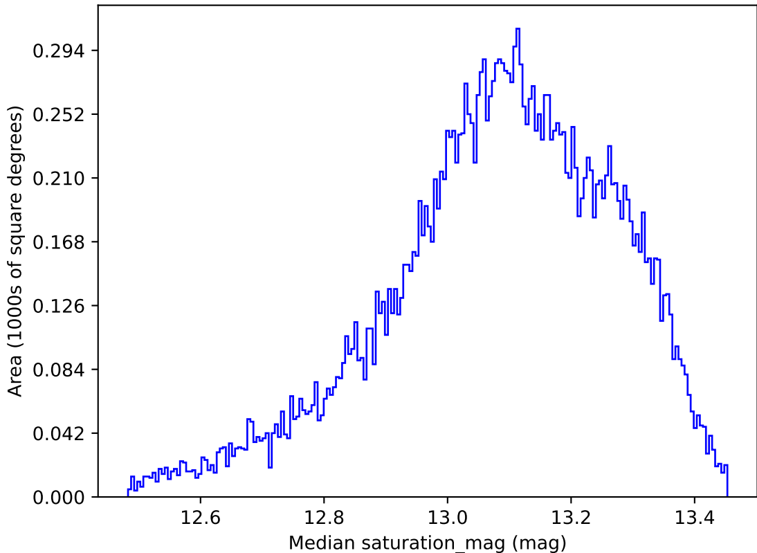
weather_cloudso0v3.5_10yrs All sky y band: Median saturation_mag
