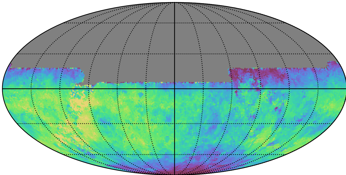
weather_cloudso0v3.5_10yrs All sky u band: Median saturation_mag
