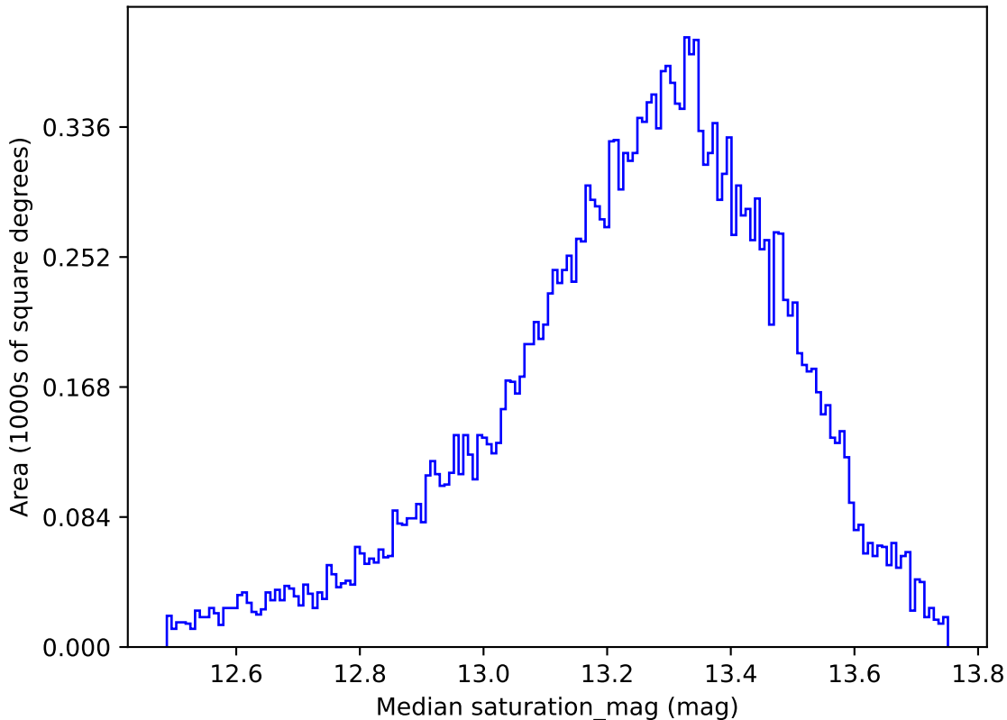
weather_cloudso0v3.5_10yrs All sky u band: Median saturation_mag
