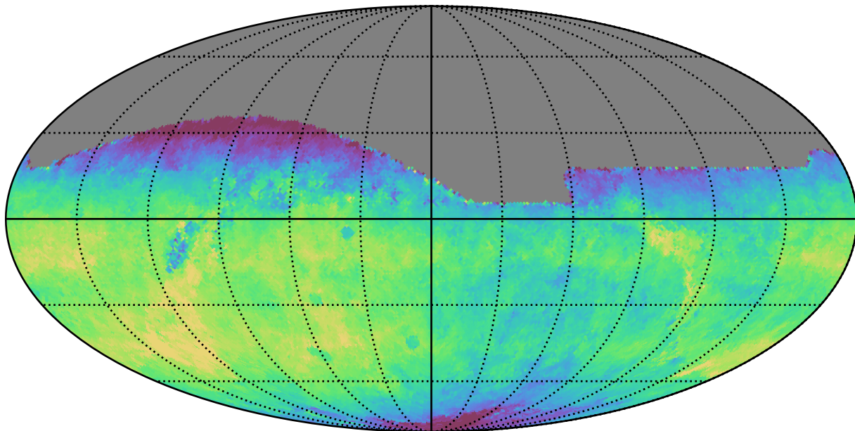
weather_cloudso0v3.5_10yrs All sky r band: Median saturation_mag
