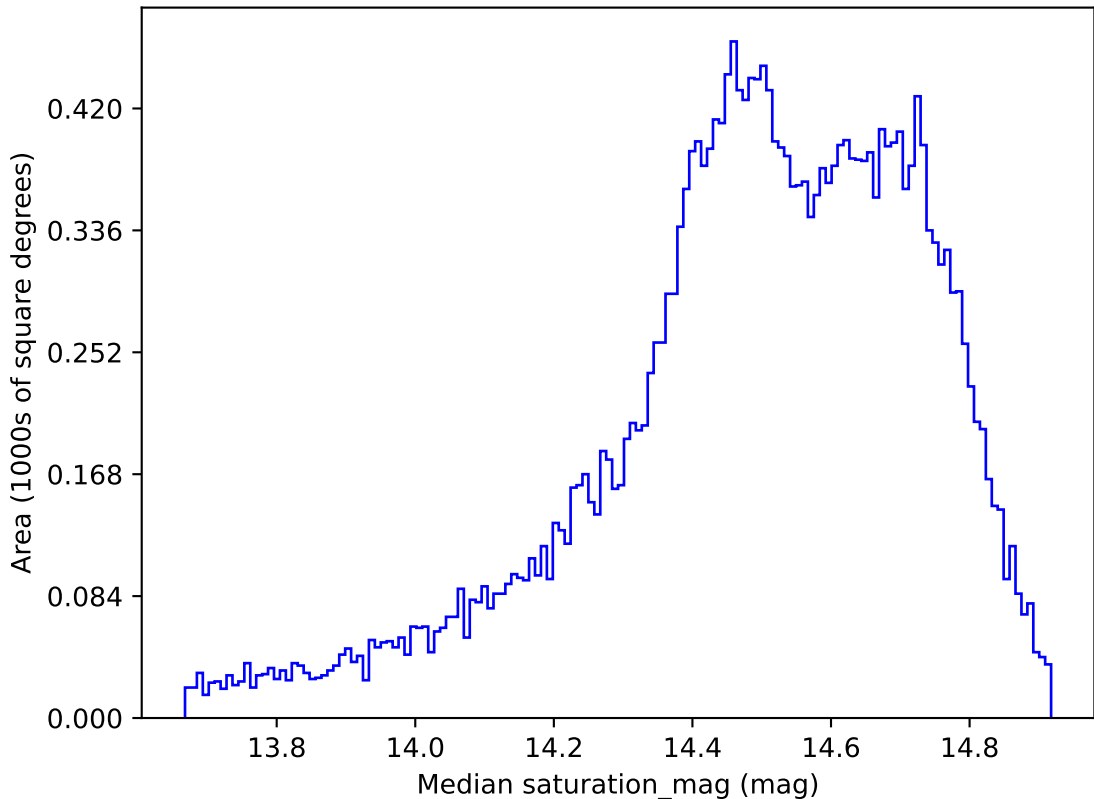
weather_cloudso0v3.5_10yrs All sky r band: Median saturation_mag
