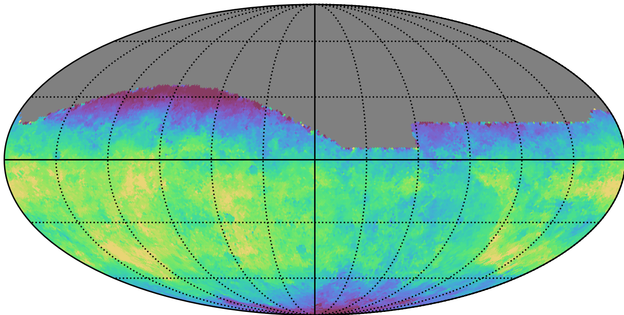
weather_cloudso0v3.5_10yrs All sky g band: Median saturation_mag
