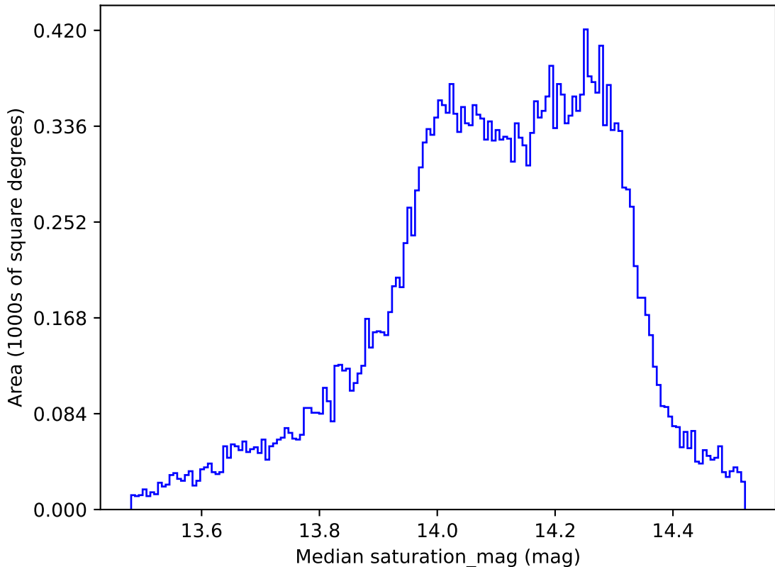
weather_cloudso0v3.5_10yrs All sky all bands: Median saturation_mag
