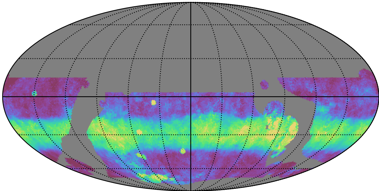
weather_cloudso0v3.5_10yrs WFD y band: Median normairmass
