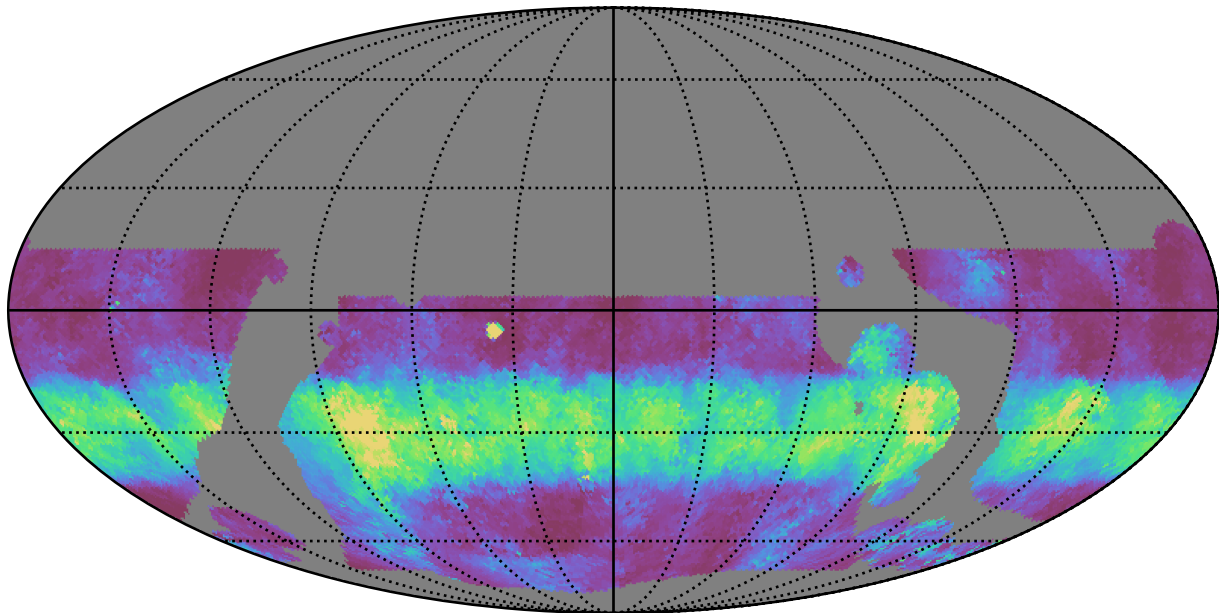
weather_cloudso0v3.5_10yrs WFD u band: Median normairmass
