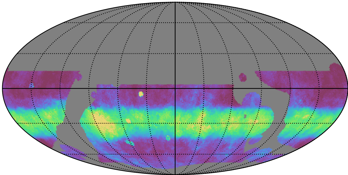
weather_cloudso0v3.5_10yrs WFD r band: Median normairmass
