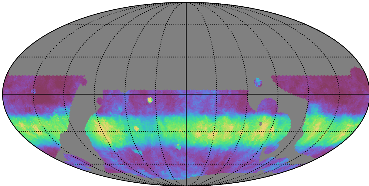
weather_cloudso0v3.5_10yrs WFD i band: Median normairmass
