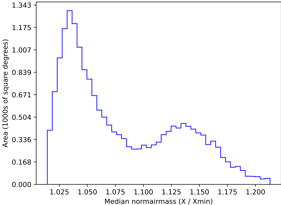
weather_cloudso0v3.5_10yrs WFD g band: Median normairmass
