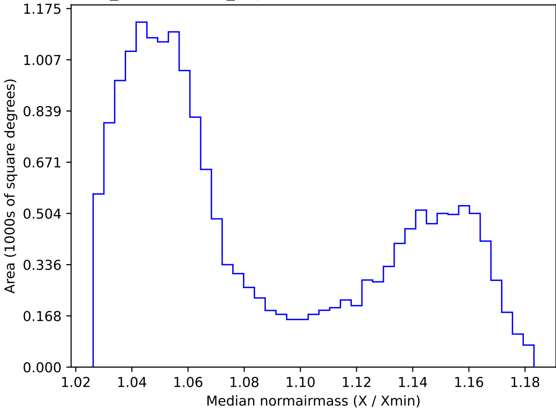
weather_cloudso0v3.5_10yrs WFD all bands: Median normairmass
