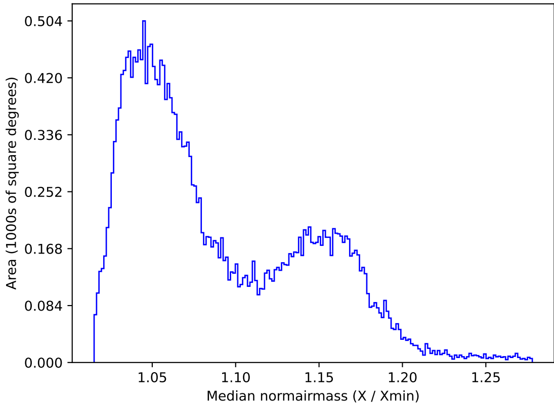
weather_cloudso0v3.5_10yrs All sky z band: Median normairmass
