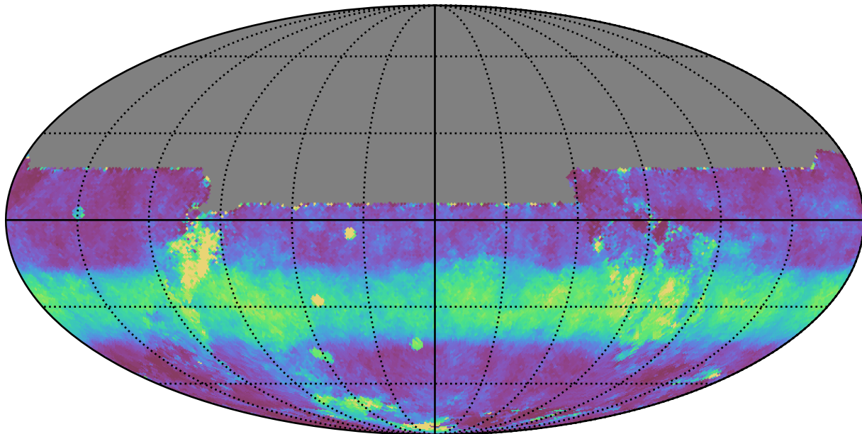
weather_cloudso0v3.5_10yrs All sky y band: Median normairmass
