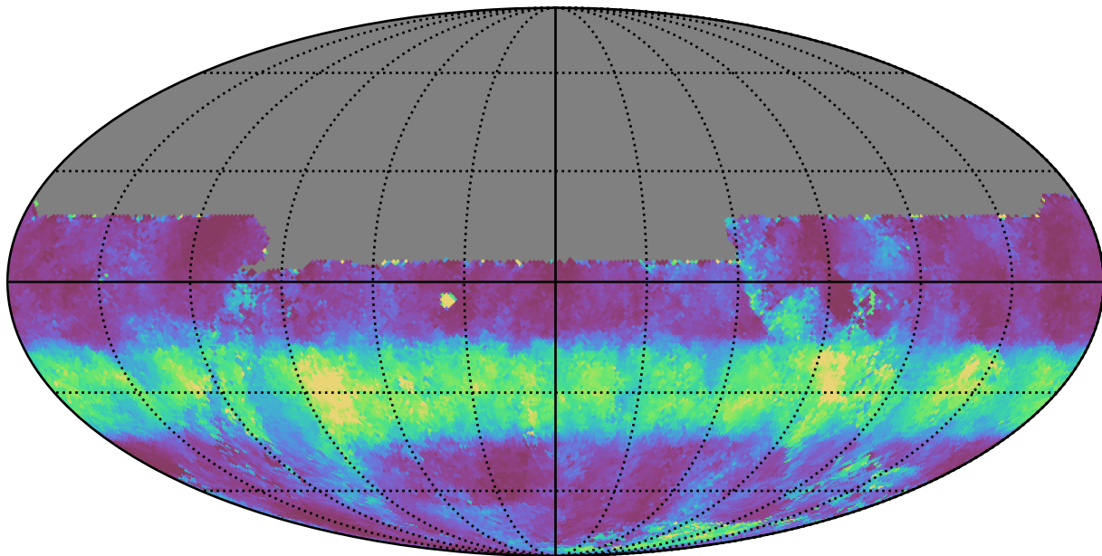
weather_cloudso0v3.5_10yrs All sky u band: Median normairmass
