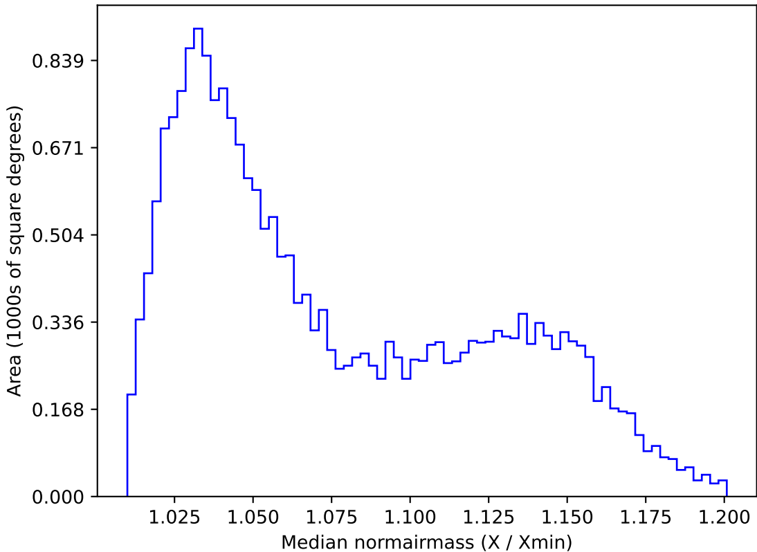
weather_cloudso0v3.5_10yrs All sky u band: Median normairmass
