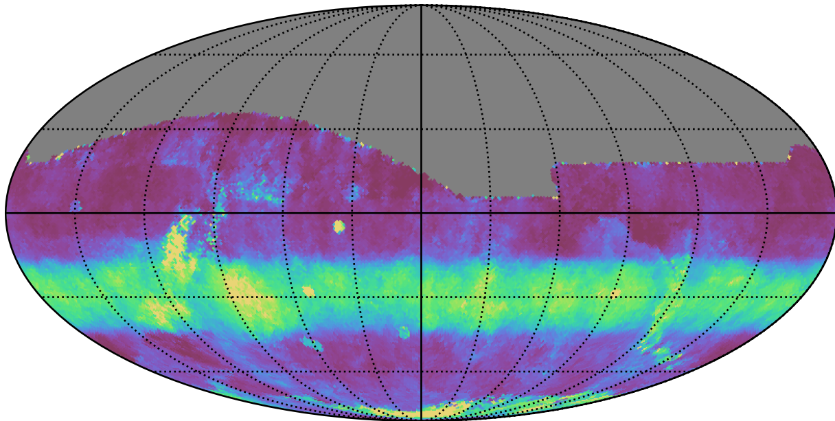
weather_cloudso0v3.5_10yrs All sky r band: Median normairmass
