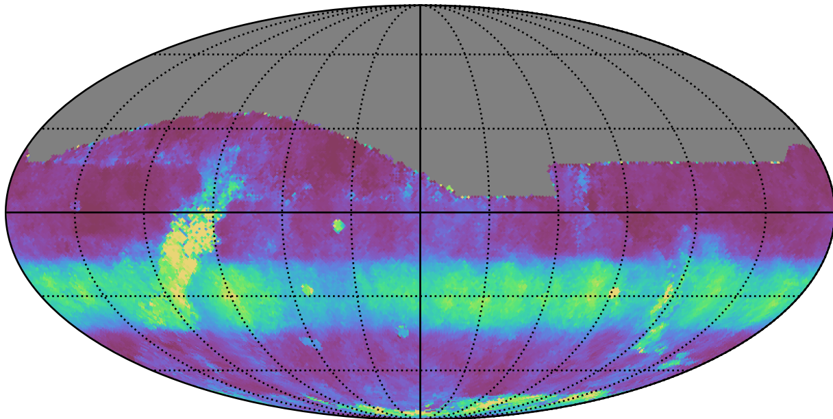
weather_cloudso0v3.5_10yrs All sky i band: Median normairmass
