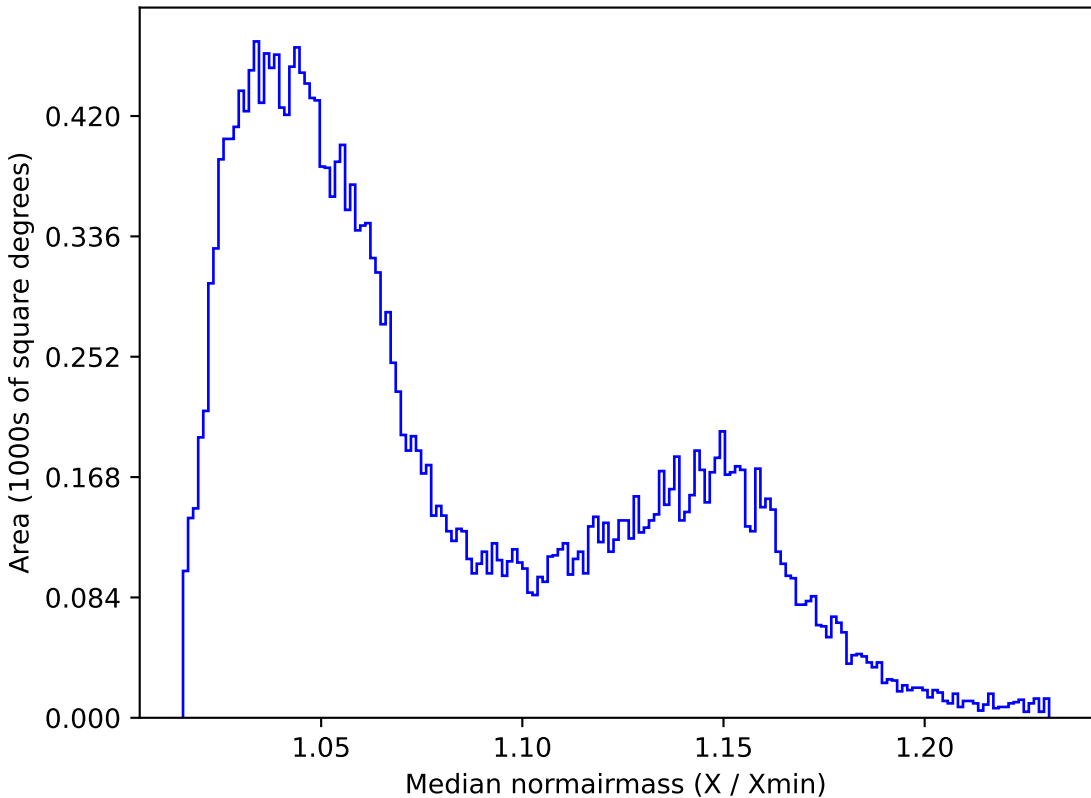
weather_cloudso0v3.5_10yrs All sky i band: Median normairmass
