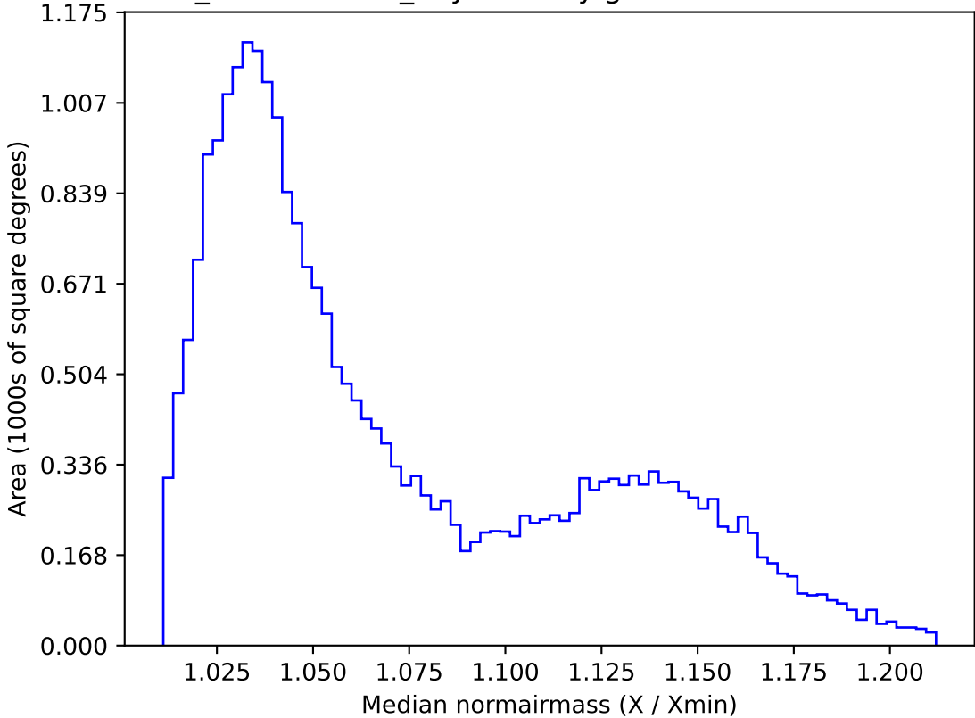
weather_cloudso0v3.5_10yrs All sky g band: Median normairmass
