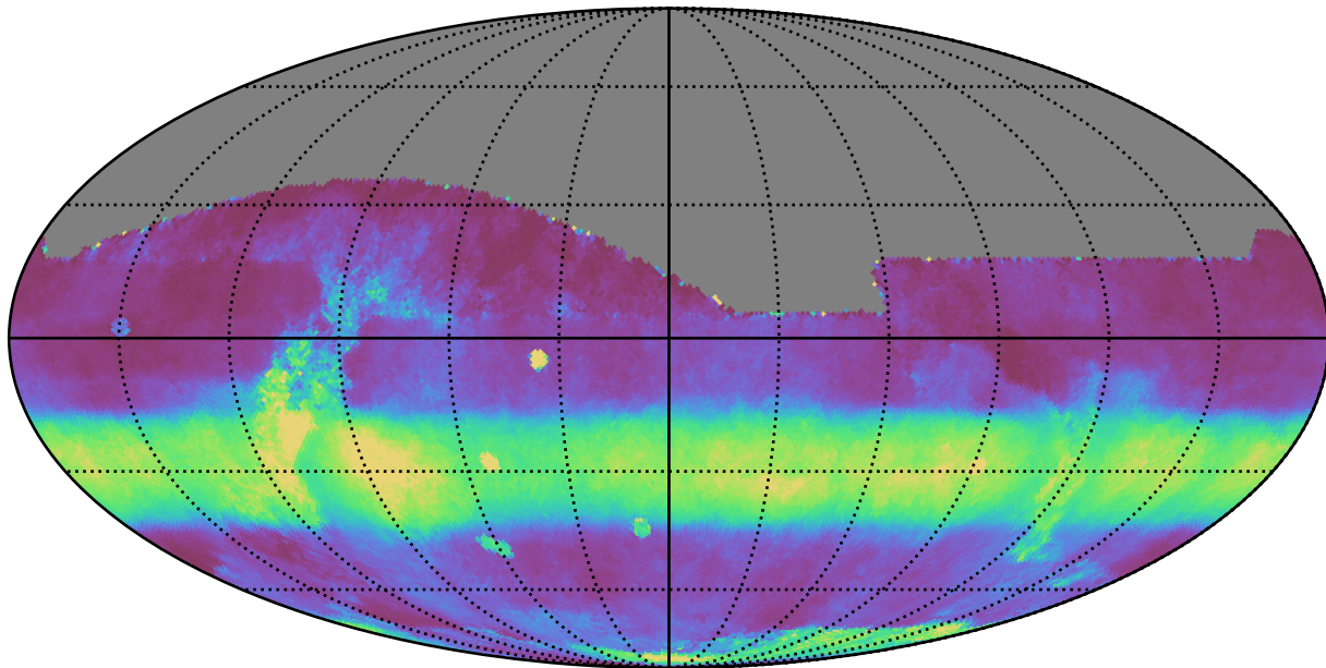
weather_cloudso0v3.5_10yrs All sky all bands: Median normairmass
