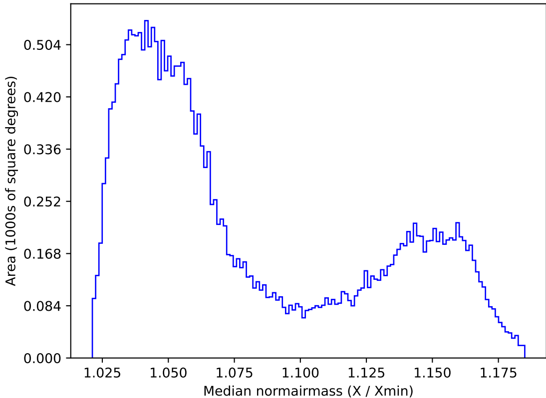
weather_cloudso0v3.5_10yrs All sky all bands: Median normairmass
