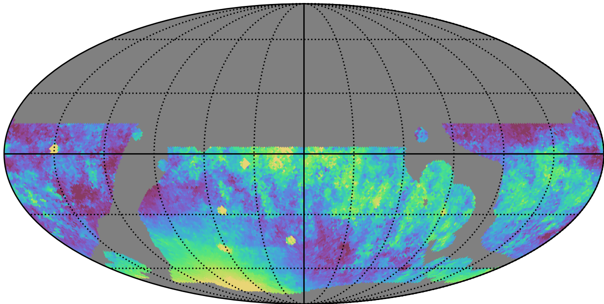
weather_cloudso0v3.5_10yrs WFD z band: Median moonDistance
