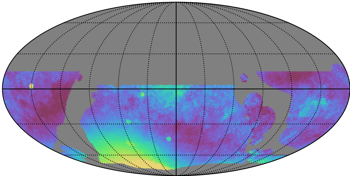
weather_cloudso0v3.5_10yrs WFD y band: Median moonDistance
