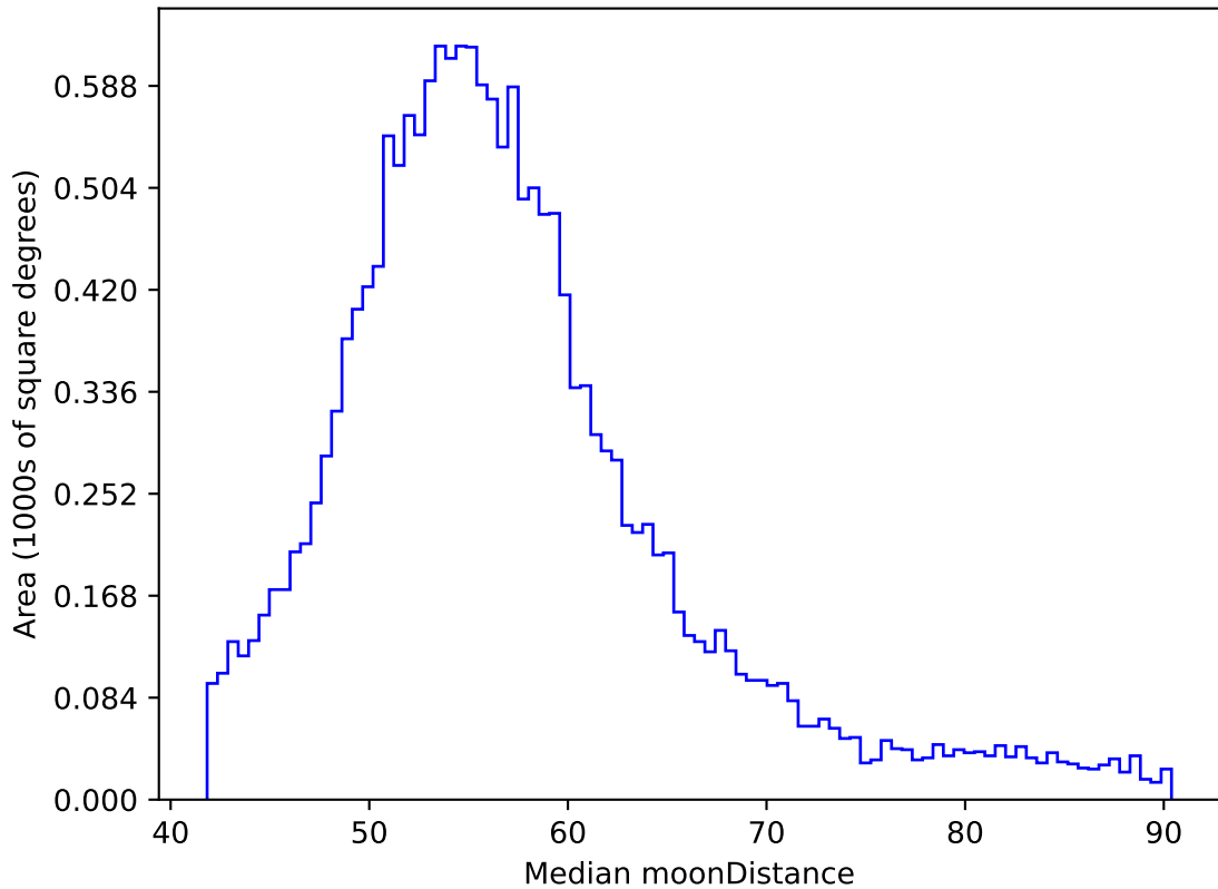
weather_cloudso0v3.5_10yrs WFD y band: Median moonDistance
