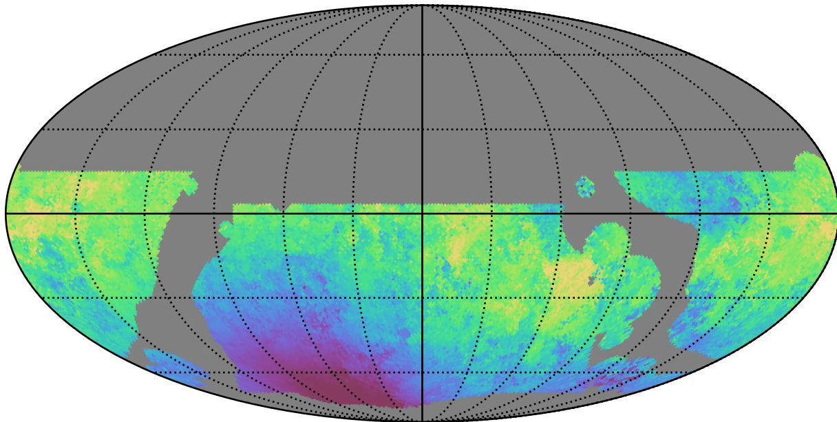
weather_cloudso0v3.5_10yrs WFD u band: Median moonDistance
